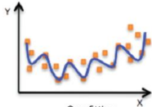
Overfitting
