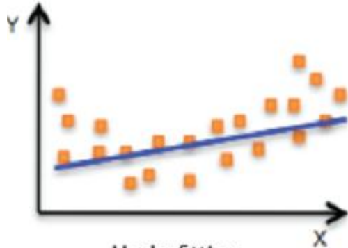
Underfitting
