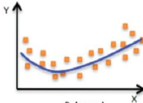
Balanced
